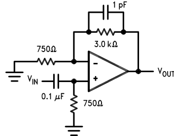
Video-Bandwidth Amplifier
